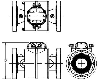
FLANGE WITH QB ELECTRONICS
