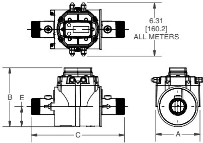
NPT / BSPP WITH 09 ELECTRONICS
